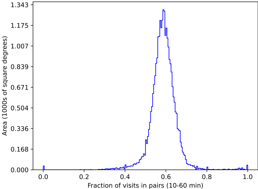
baseline_v3.0_10yrs gri All sky: Fraction of visits in pairs (10-60 min)
