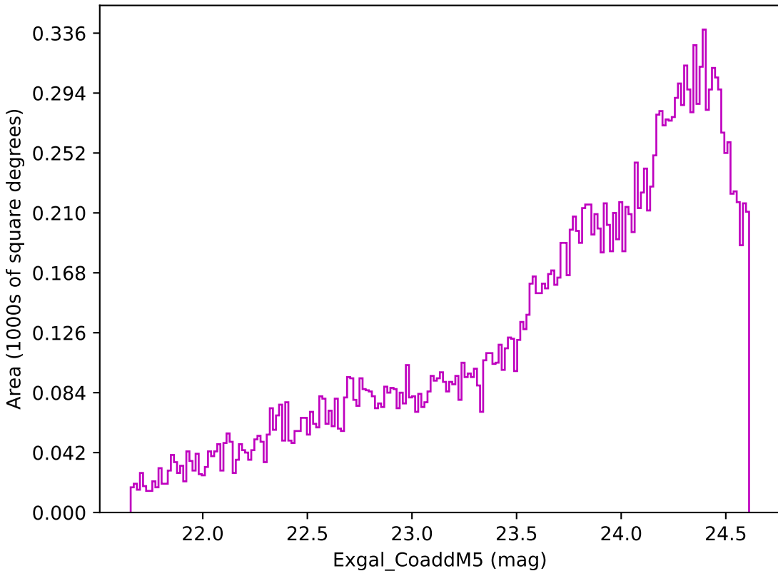
baseline_v3.0_10yrs Yr 3-4 z band: Exgal_CoaddM5
