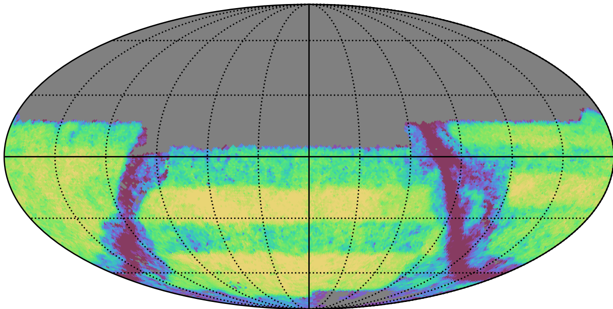
baseline_v3.0_10yrs Yr 3-4 y band: Exgal_CoaddM5
