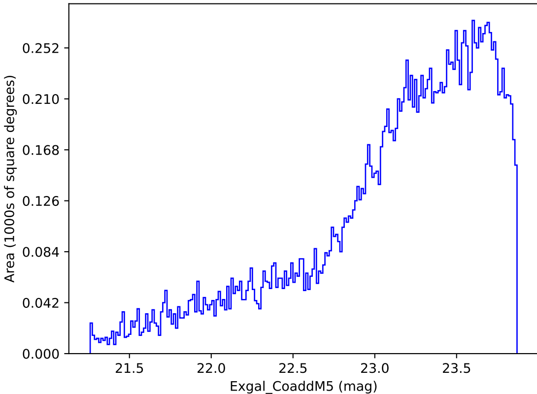
baseline_v3.0_10yrs Yr 3-4 y band: Exgal_CoaddM5
