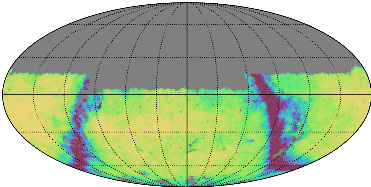
baseline_v3.0_10yrs Yr 3-4 u band: Exgal_CoaddM5
