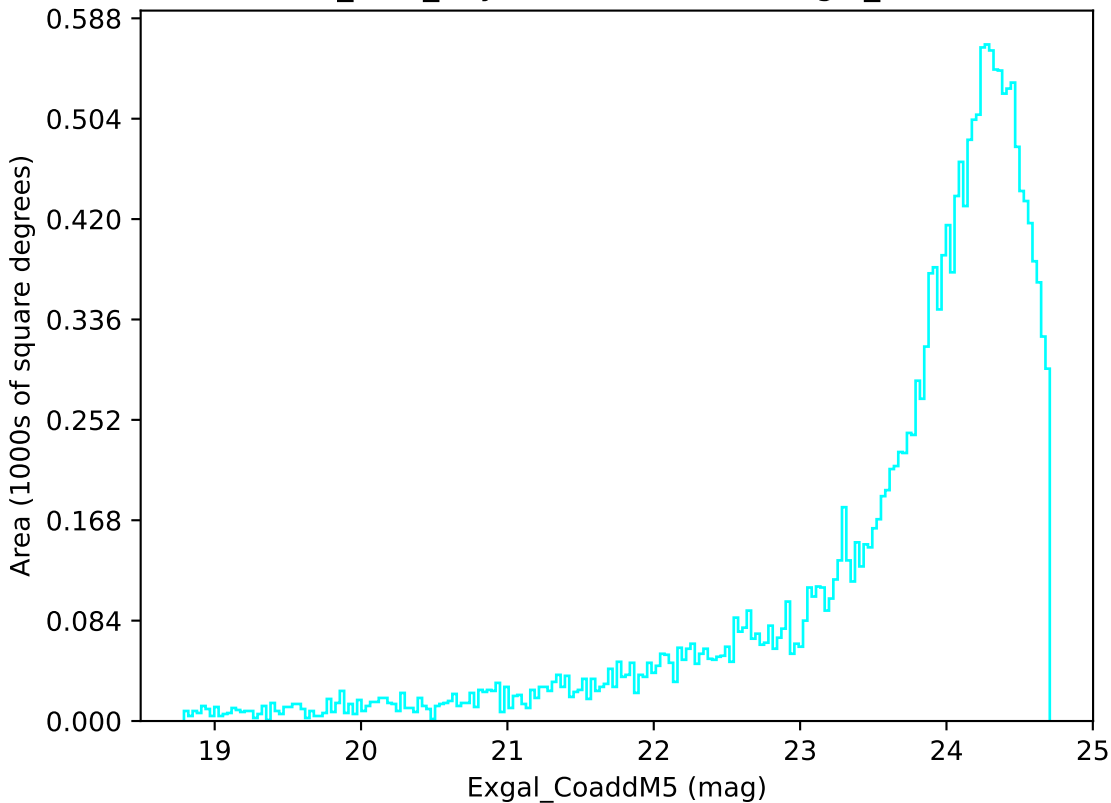
baseline_v3.0_10yrs Yr 3-4 u band: Exgal_CoaddM5
