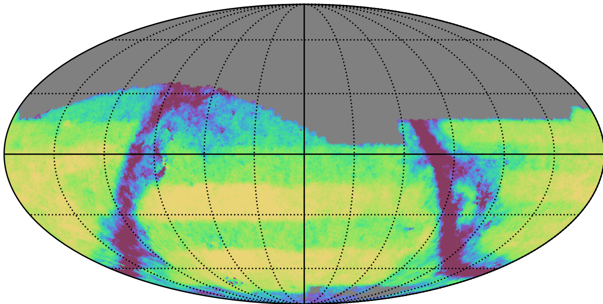
baseline_v3.0_10yrs Yr 3-4 r band: Exgal_CoaddM5
