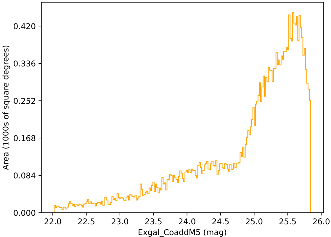
baseline_v3.0_10yrs Yr 3-4 r band: Exgal_CoaddM5
