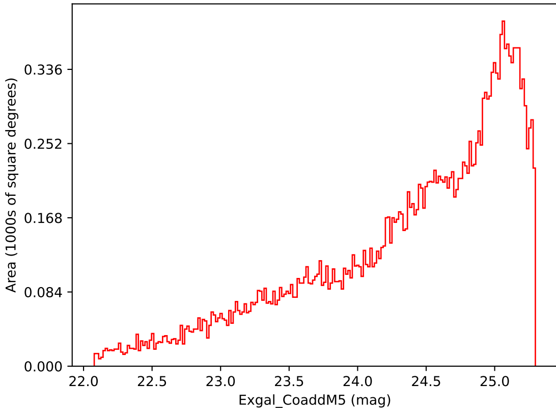
baseline_v3.0_10yrs Yr 3-4 i band: Exgal_CoaddM5
