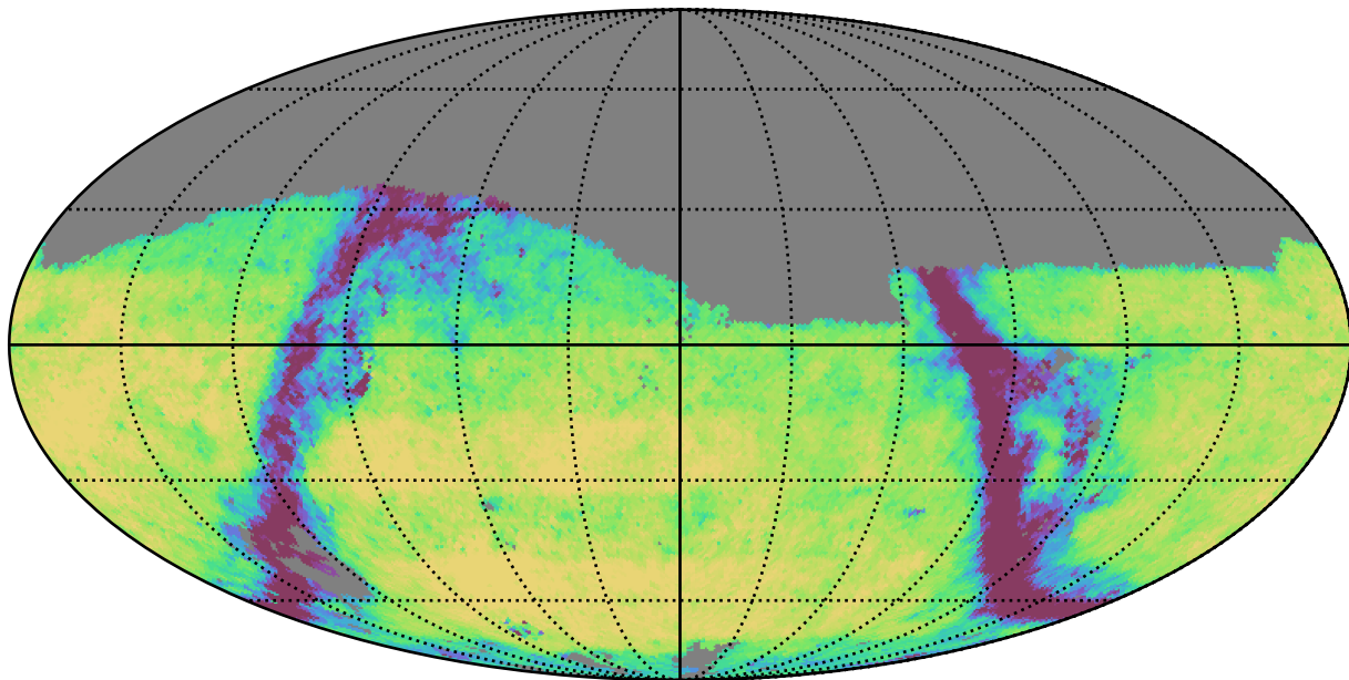
baseline_v3.0_10yrs Yr 3-4 g band: Exgal_CoaddM5
