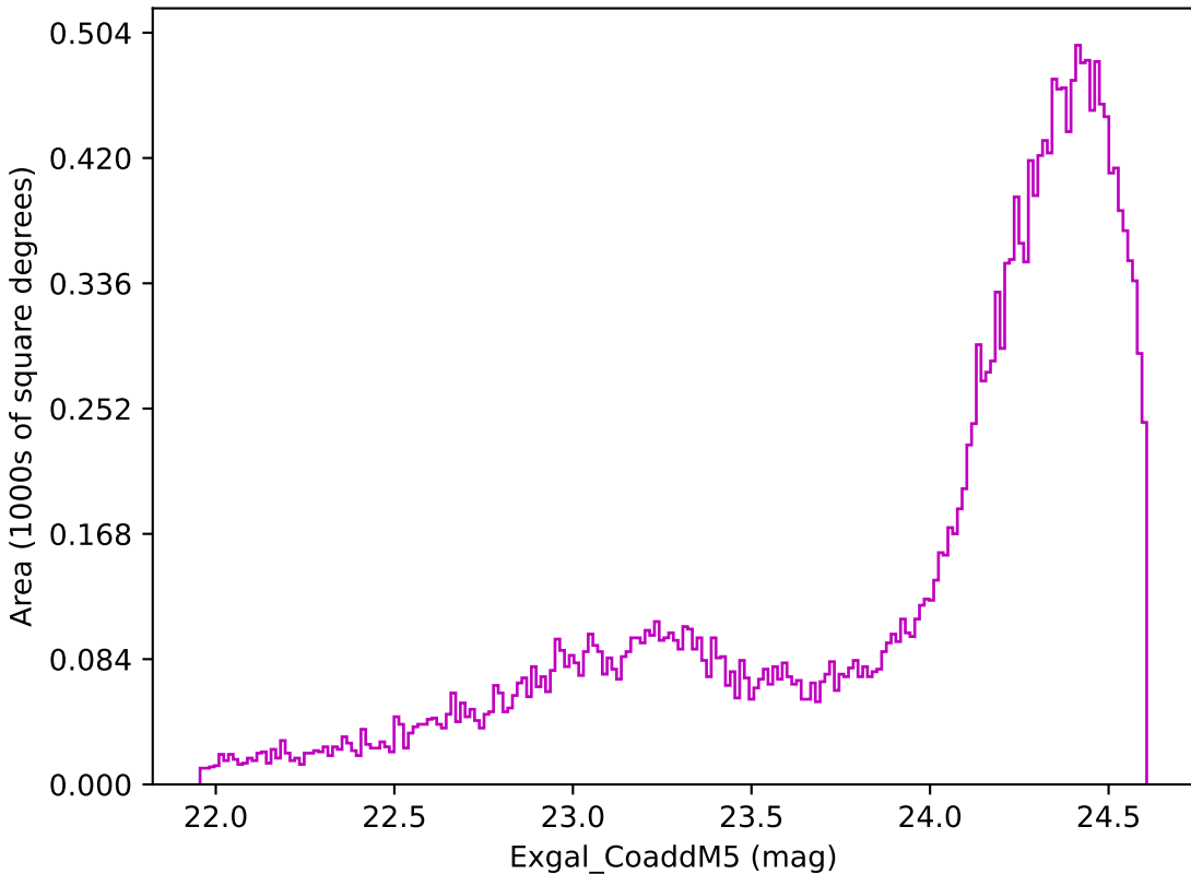
baseline_v3.0_10yrs Yr 1 z band: Exgal_CoaddM5
