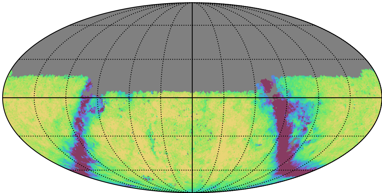
baseline_v3.0_10yrs Yr 1 u band: Exgal_CoaddM5
