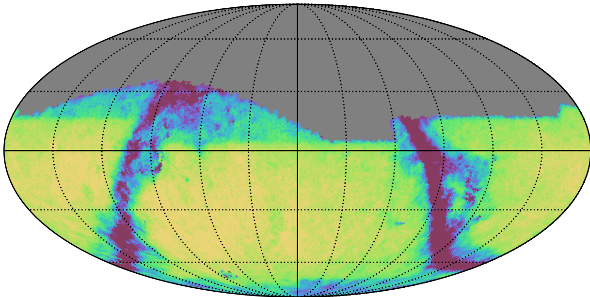
baseline_v3.0_10yrs Yr 1 r band: Exgal_CoaddM5
