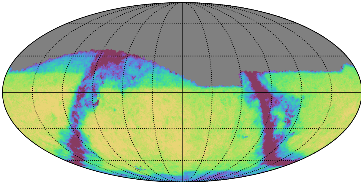
baseline_v3.0_10yrs Yr 1 i band: Exgal_CoaddM5
