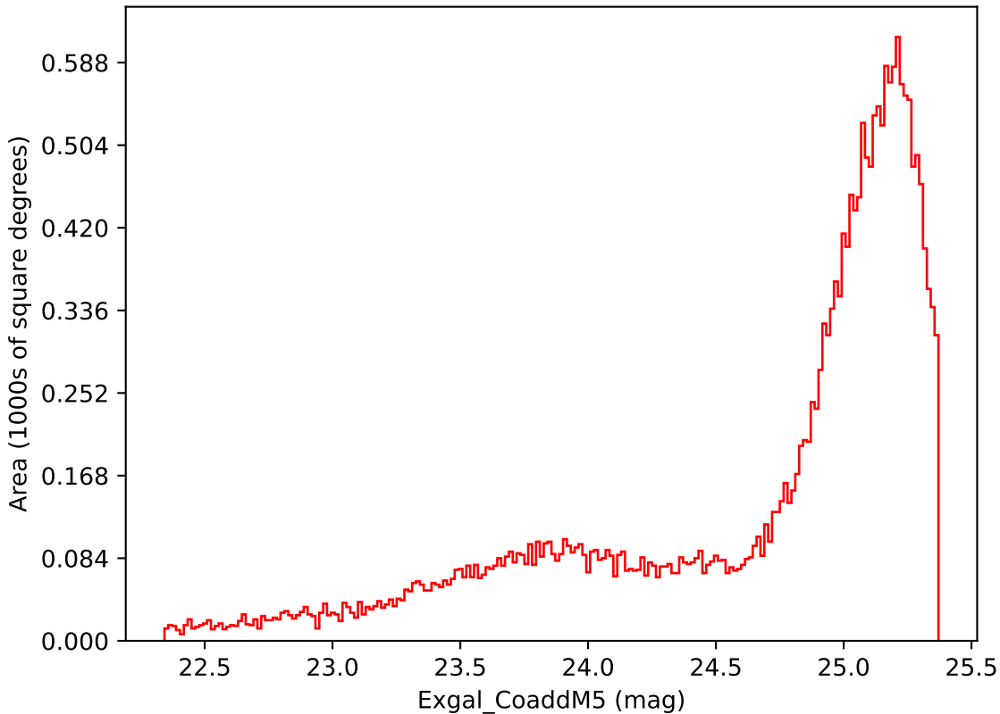
baseline_v3.0_10yrs Yr 1 i band: Exgal_CoaddM5
