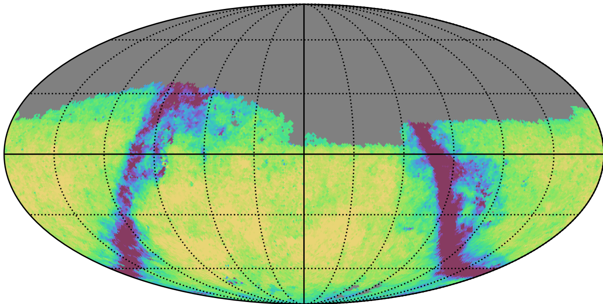
baseline_v3.0_10yrs Yr 1 g band: Exgal_CoaddM5
