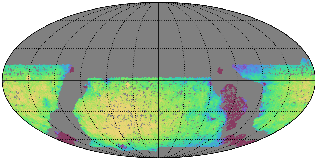
baseline_v3.0_10yrs WFD z band: Exgal_CoaddM5
