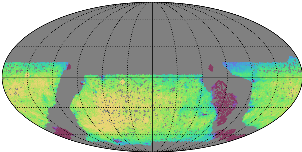
baseline_v3.0_10yrs WFD y band: Exgal_CoaddM5
