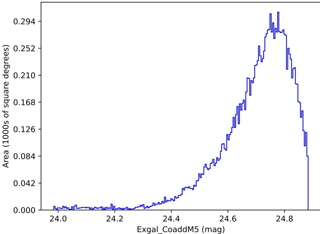
baseline_v3.0_10yrs WFD y band: Exgal_CoaddM5
