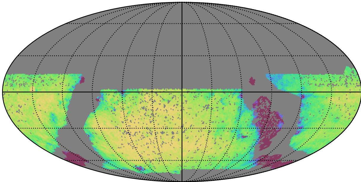
baseline_v3.0_10yrs WFD u band: Exgal_CoaddM5
