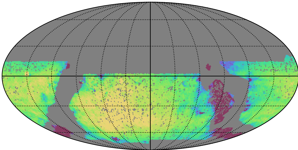
baseline_v3.0_10yrs WFD r band: Exgal_CoaddM5
