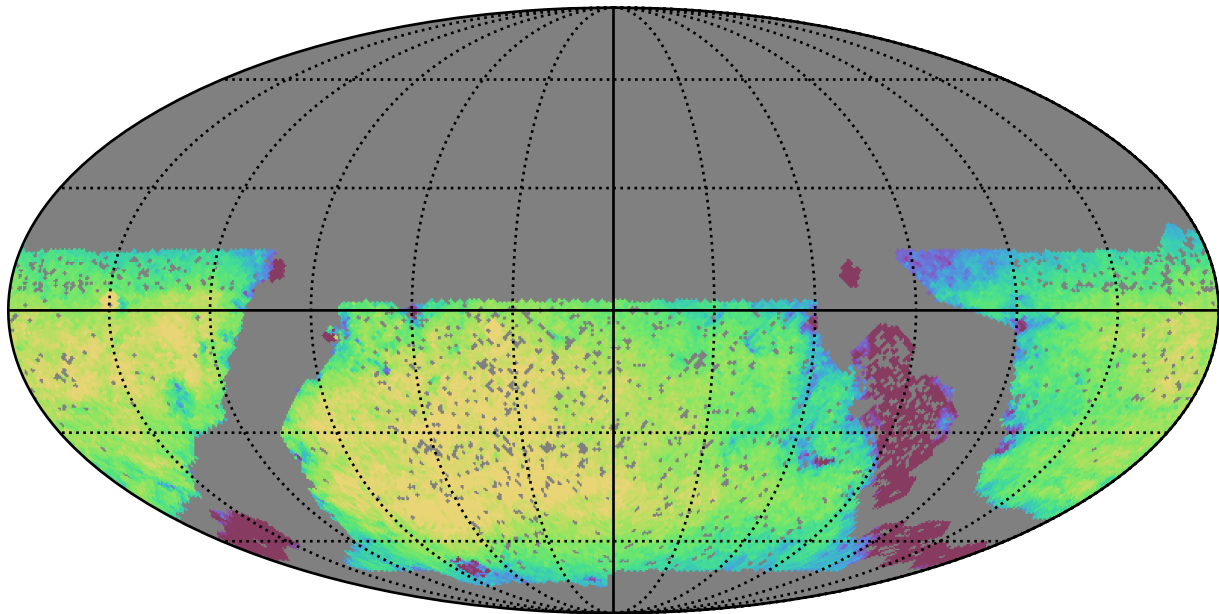
baseline_v3.0_10yrs WFD i band: Exgal_CoaddM5
