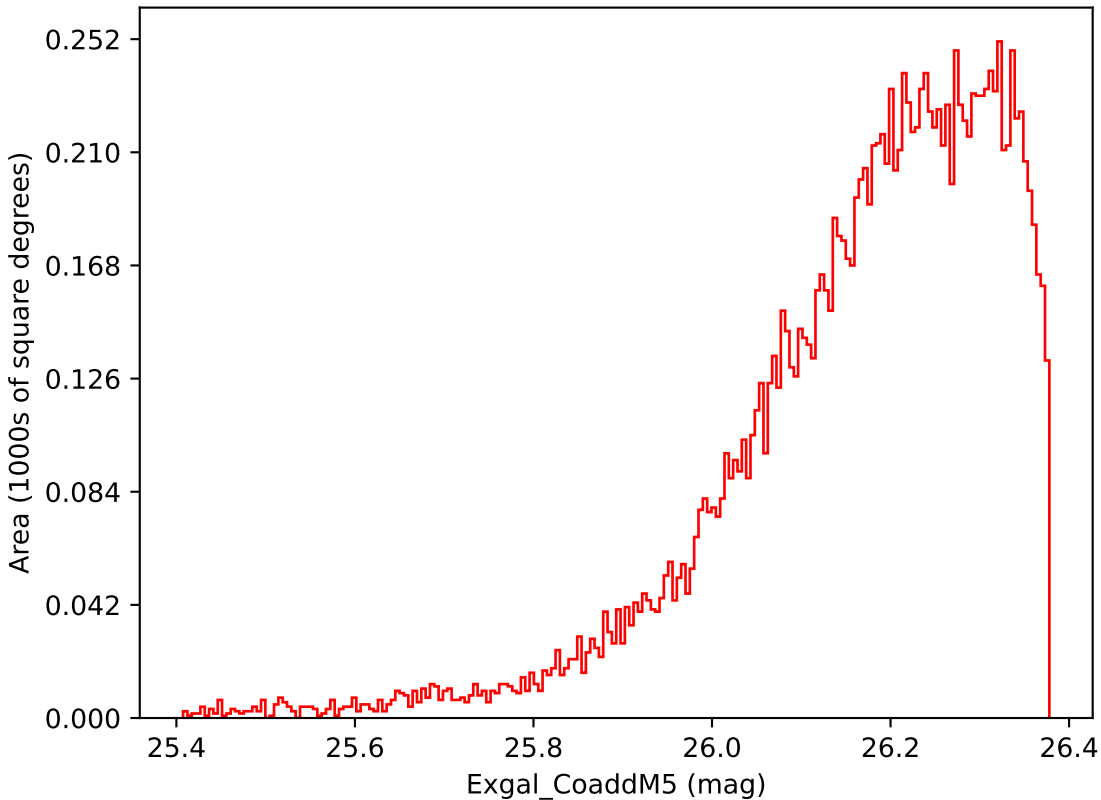
baseline_v3.0_10yrs WFD i band: Exgal_CoaddM5
