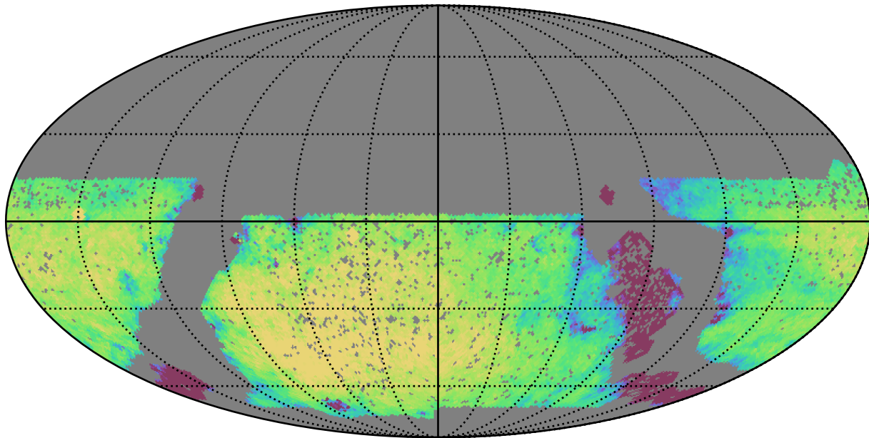
baseline_v3.0_10yrs WFD g band: Exgal_CoaddM5
