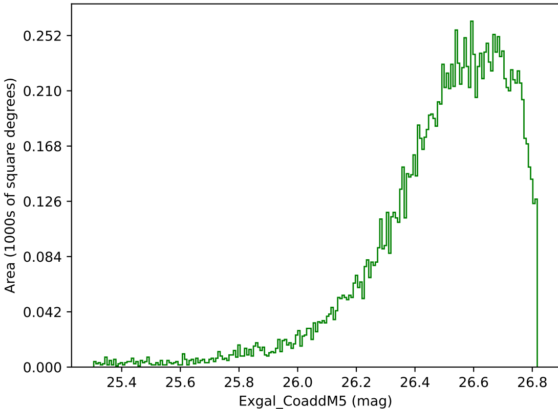
baseline_v3.0_10yrs WFD g band: Exgal_CoaddM5
