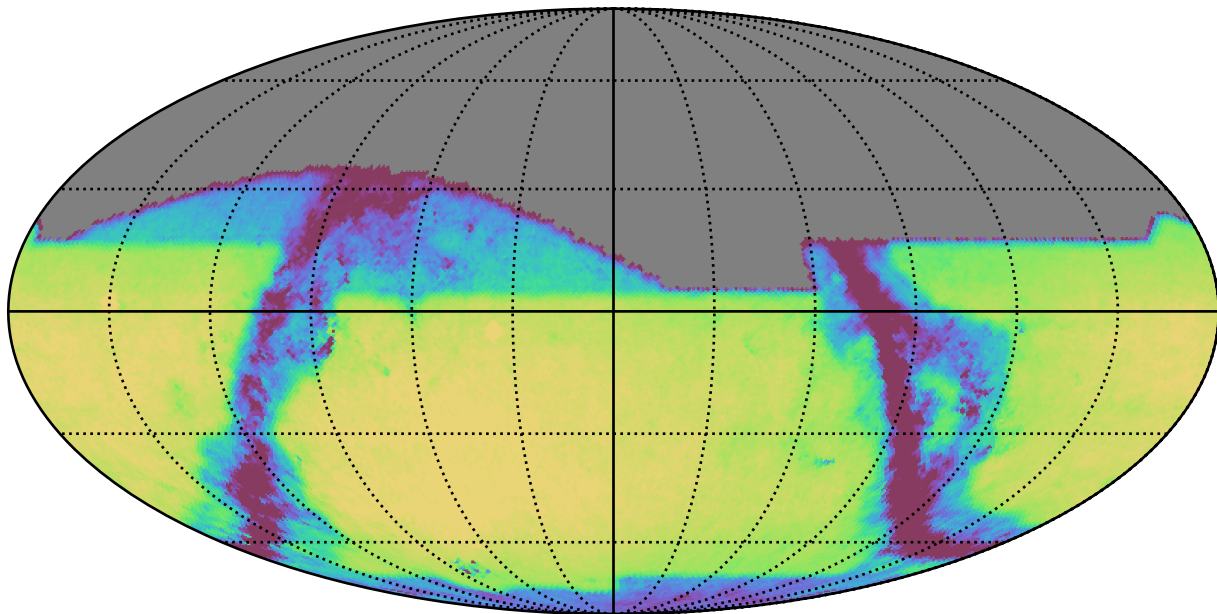
baseline_v3.0_10yrs All sky z band: Exgal_CoaddM5
