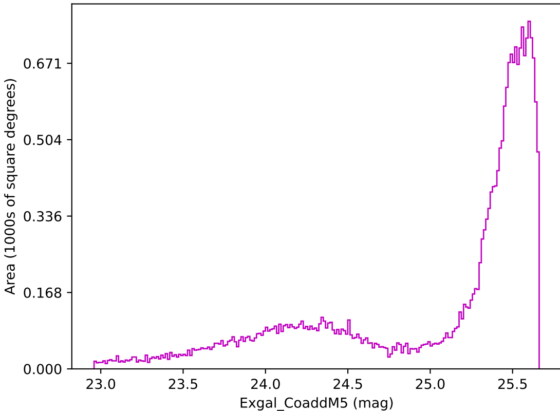
baseline_v3.0_10yrs All sky z band: Exgal_CoaddM5
