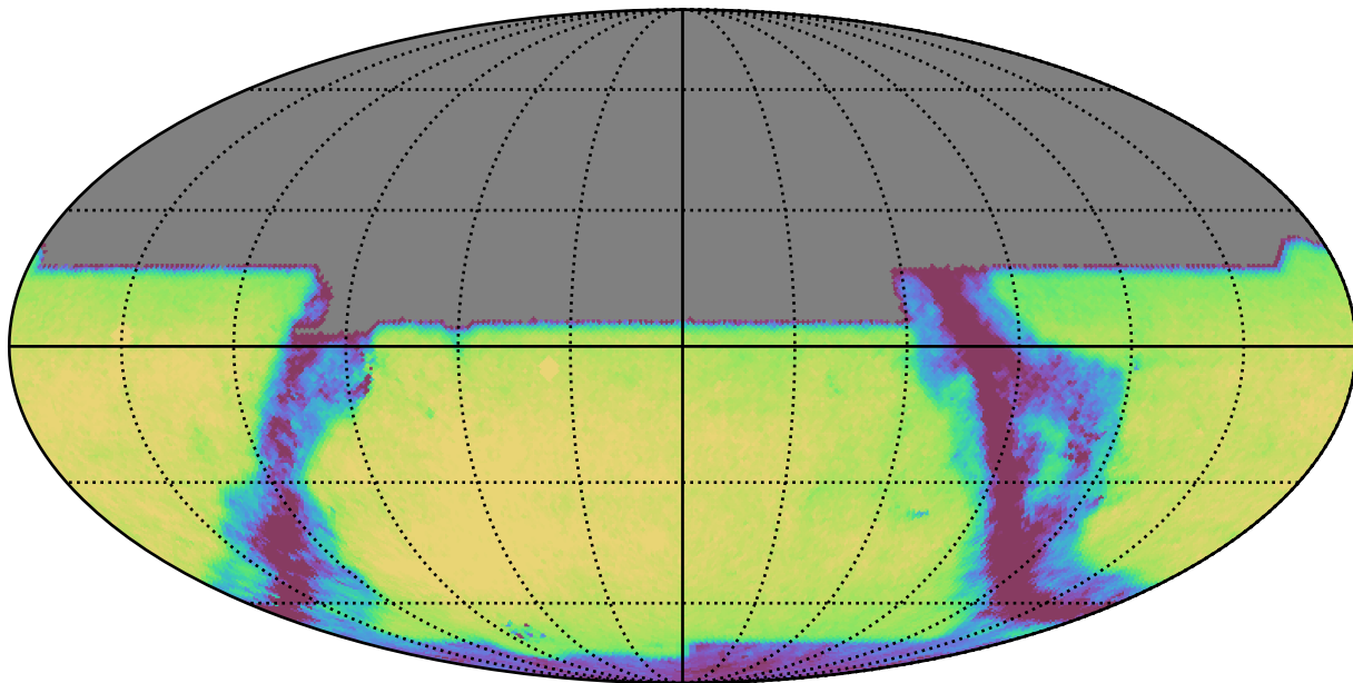
baseline_v3.0_10yrs All sky y band: Exgal_CoaddM5
