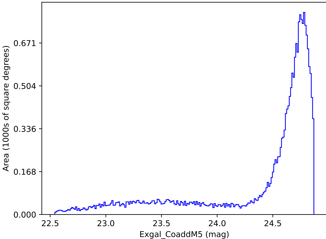
baseline_v3.0_10yrs All sky y band: Exgal_CoaddM5
