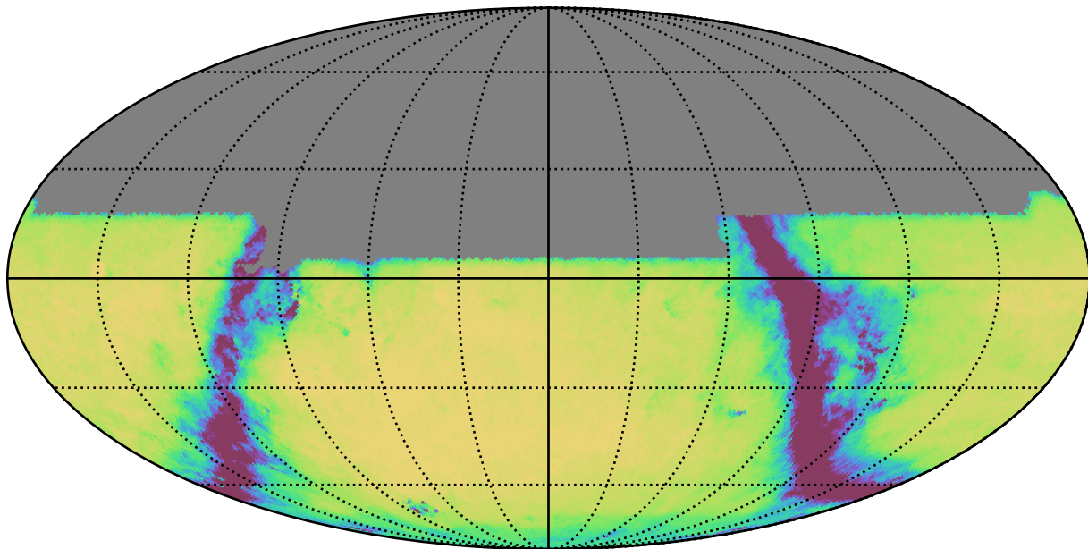
baseline_v3.0_10yrs All sky u band: Exgal_CoaddM5
