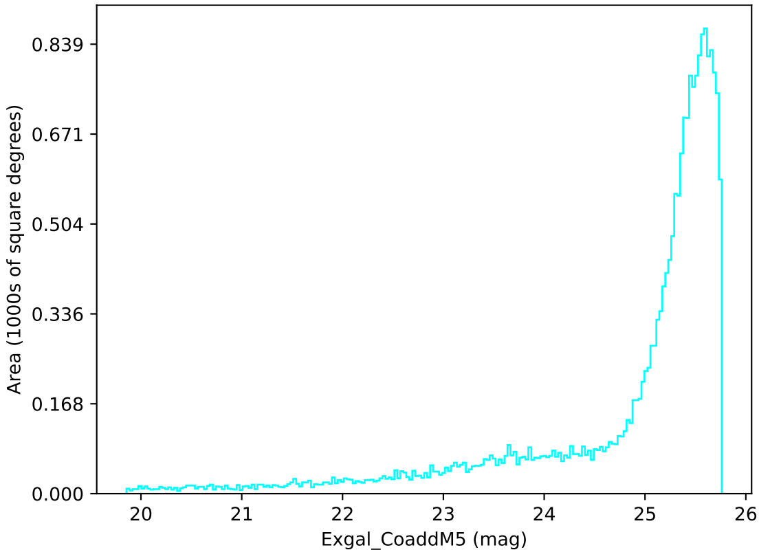
baseline_v3.0_10yrs All sky u band: Exgal_CoaddM5
