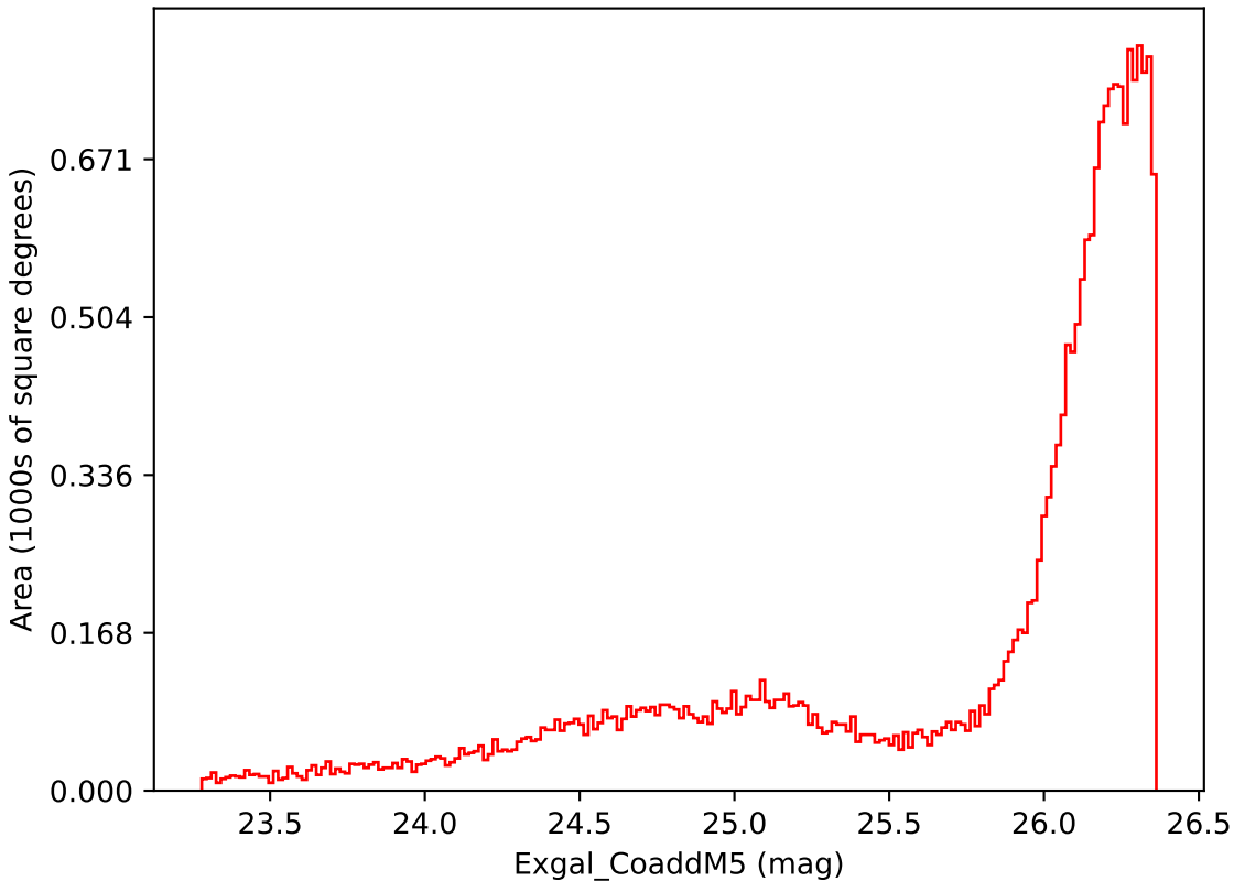
baseline_v3.0_10yrs All sky i band: Exgal_CoaddM5
