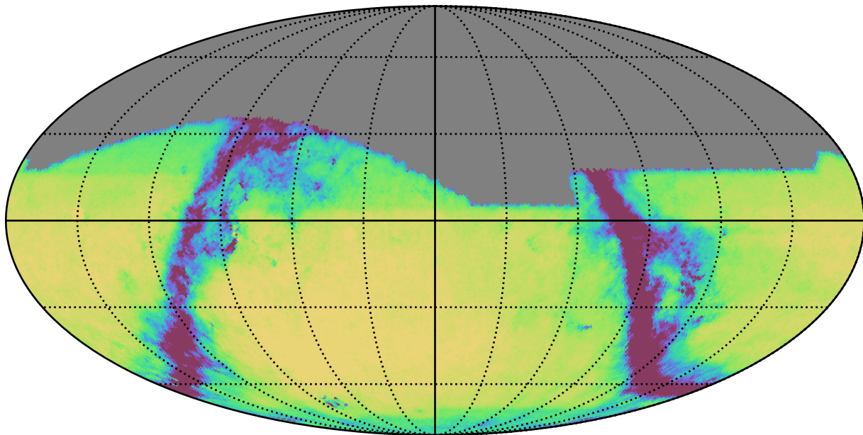
baseline_v3.0_10yrs All sky g band: Exgal_CoaddM5
