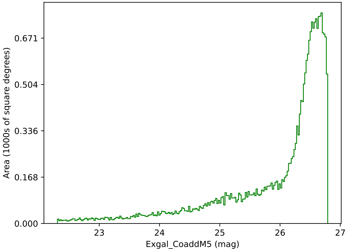
baseline_v3.0_10yrs All sky g band: Exgal_CoaddM5
