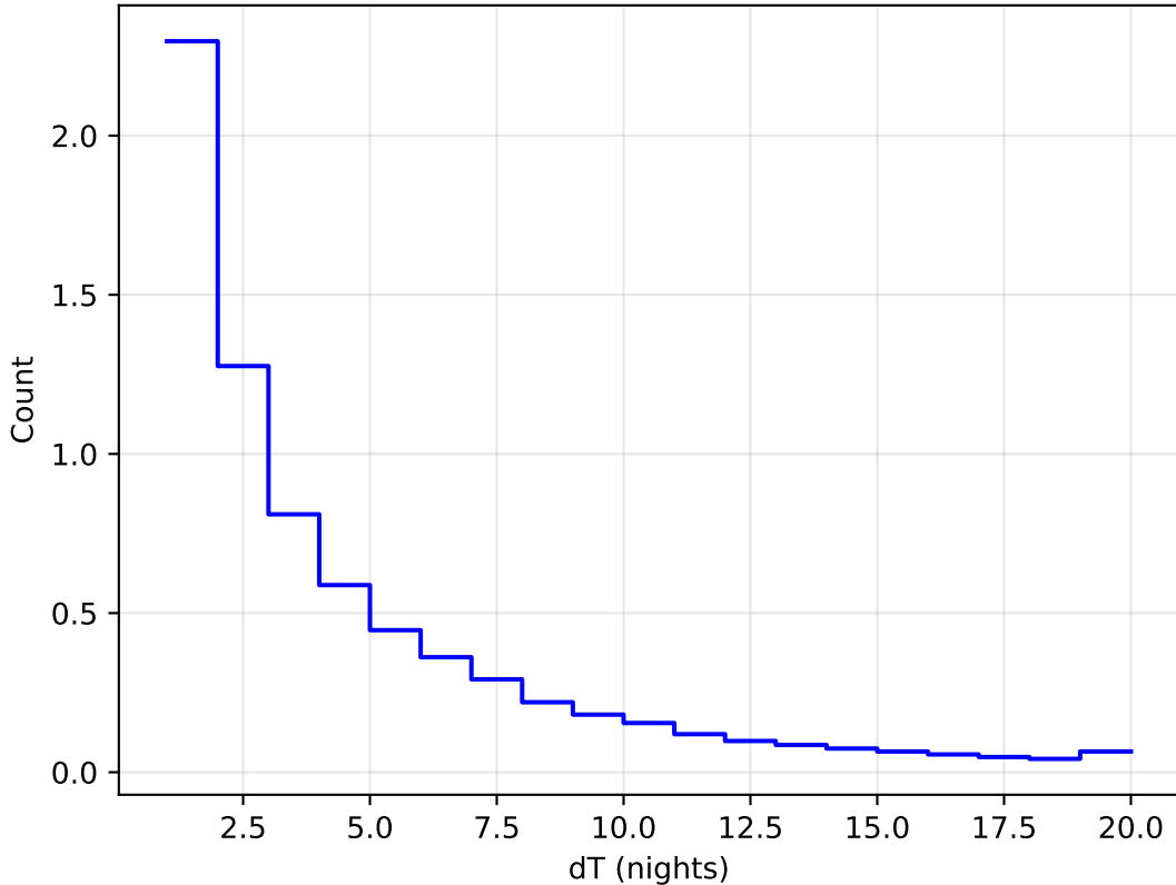
baseline_v3.0_10yrs WFD all bands: DeltaNight Histogram 1e6
