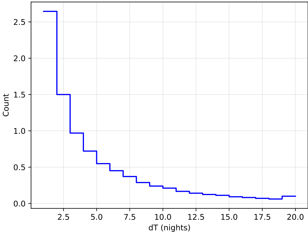
baseline_v3.0_10yrs All sky all bands: DeltaNight Histogram 1e6
