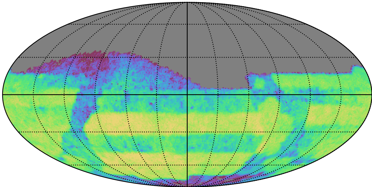
baseline_v3.0_10yrs Yr 3-4 z band: CoaddM5
