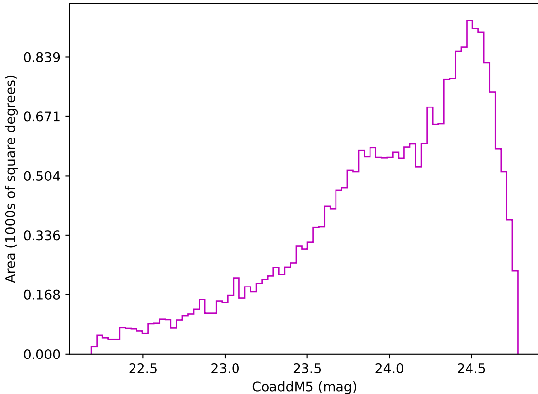
baseline_v3.0_10yrs Yr 3-4 z band: CoaddM5
