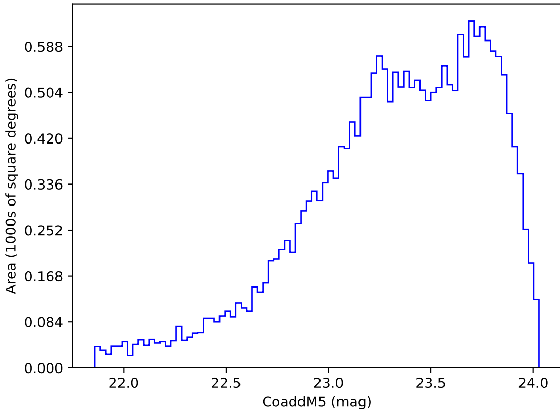
baseline_v3.0_10yrs Yr 3-4 y band: CoaddM5
