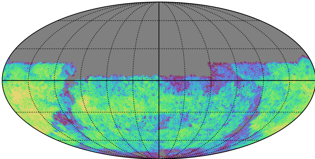
baseline_v3.0_10yrs Yr 3-4 u band: CoaddM5
