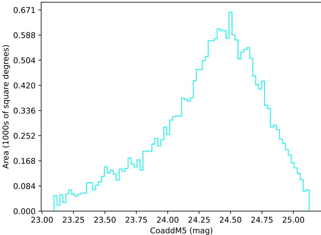
baseline_v3.0_10yrs Yr 3-4 u band: CoaddM5
