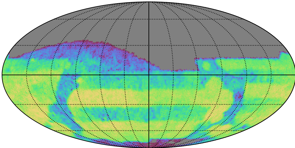
baseline_v3.0_10yrs Yr 3-4 r band: CoaddM5
