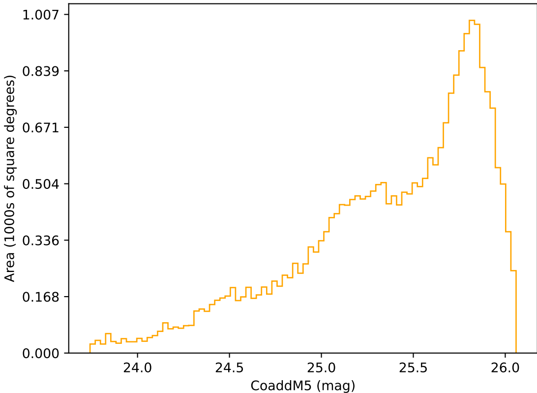
baseline_v3.0_10yrs Yr 3-4 r band: CoaddM5
