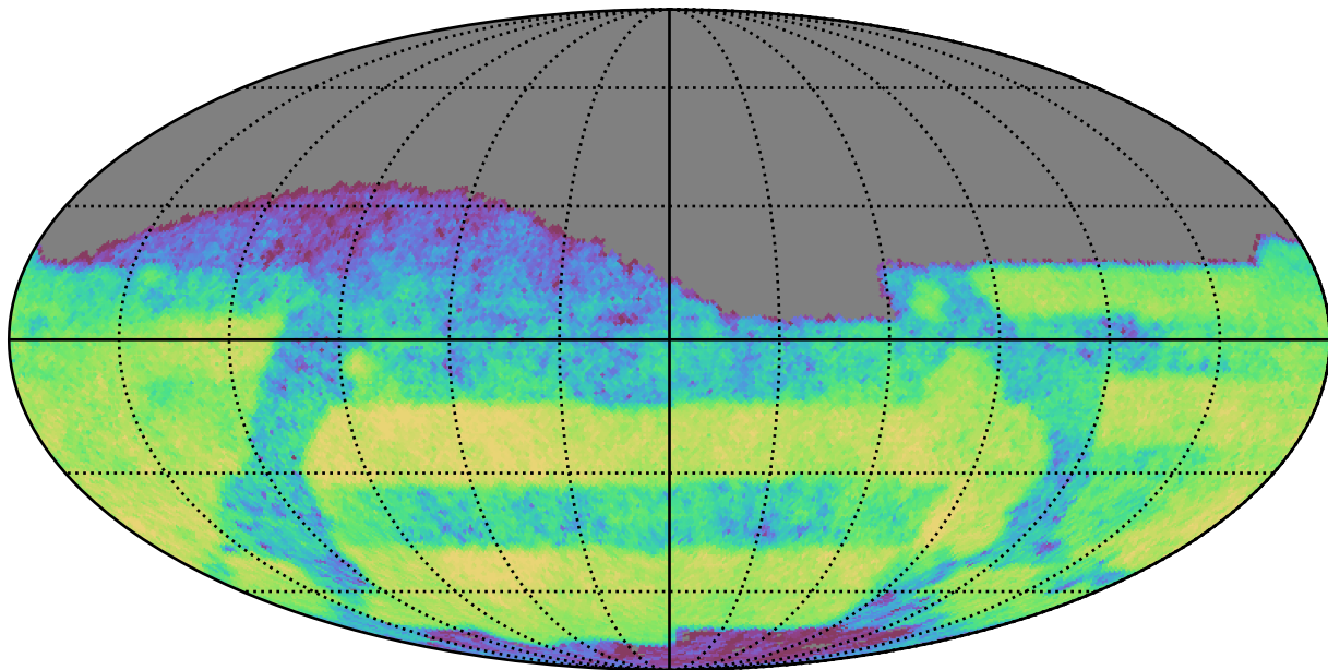
baseline_v3.0_10yrs Yr 3-4 i band: CoaddM5
