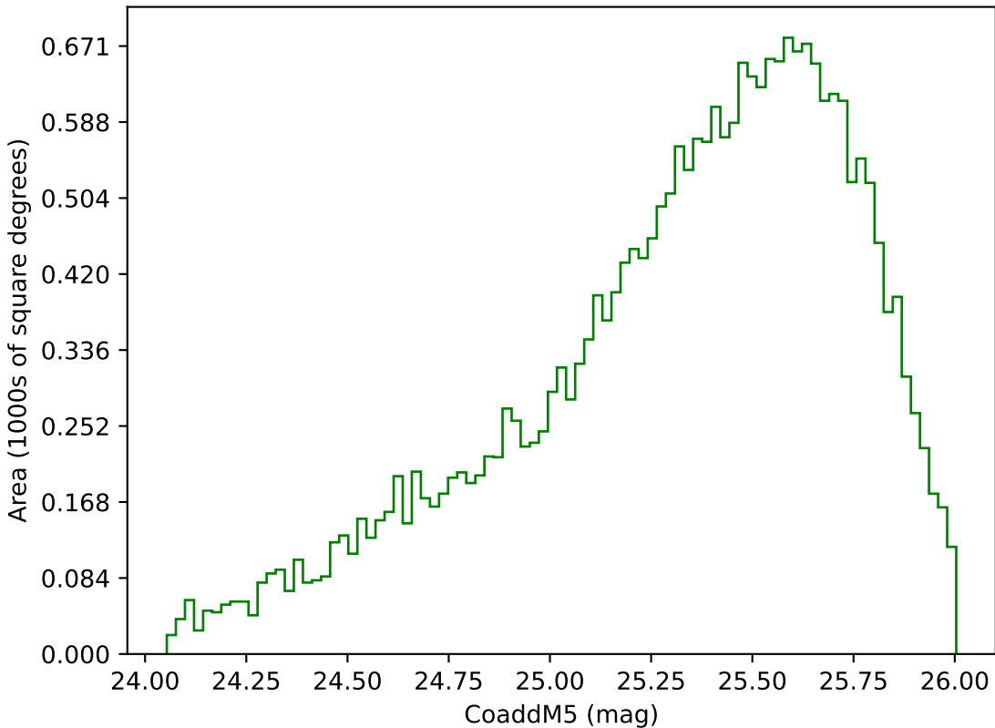
baseline_v3.0_10yrs Yr 3-4 g band: CoaddM5
