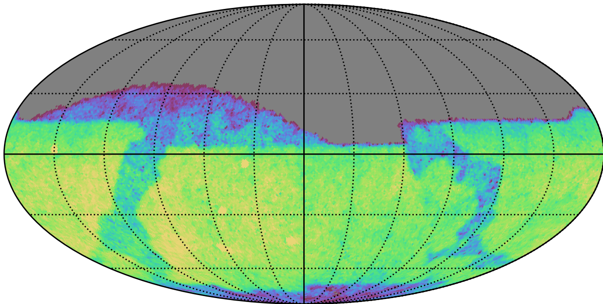
baseline_v3.0_10yrs Yr 1 z band: CoaddM5
