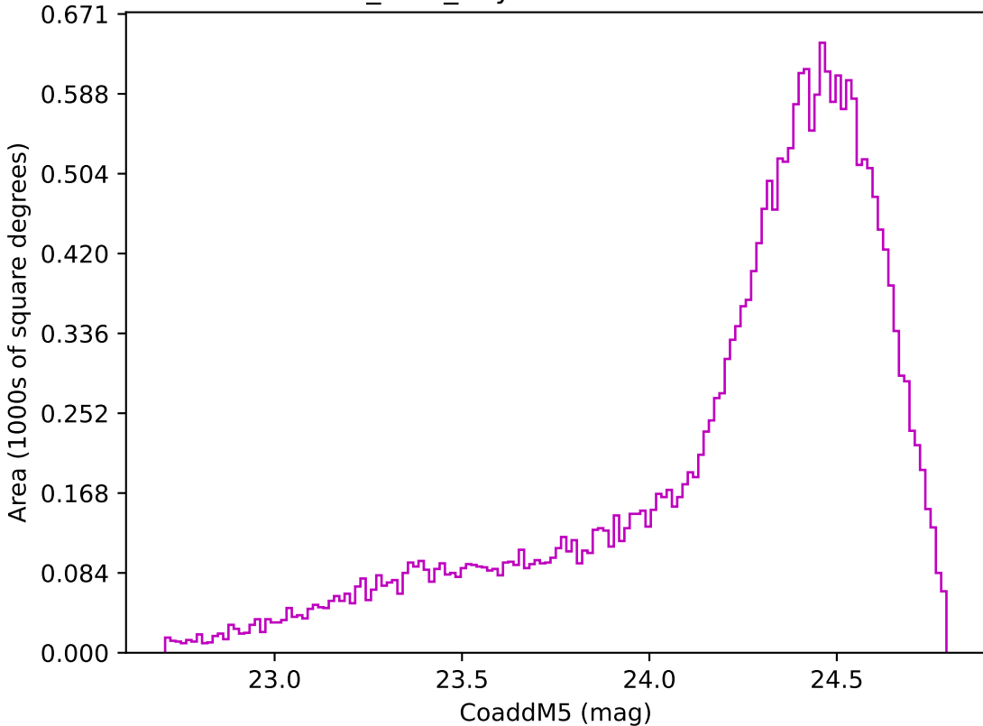
baseline_v3.0_10yrs Yr 1 z band: CoaddM5
