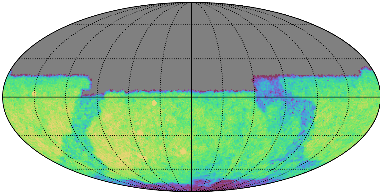
baseline_v3.0_10yrs Yr 1 y band: CoaddM5
