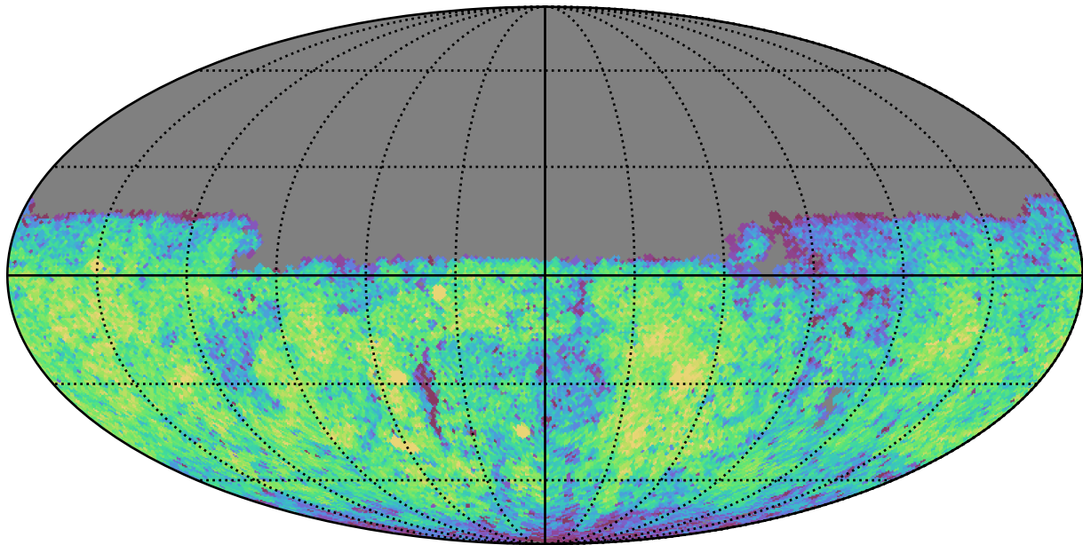
baseline_v3.0_10yrs Yr 1 u band: CoaddM5
