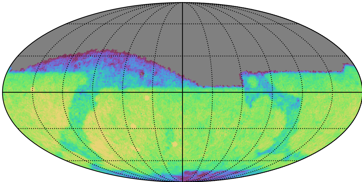
baseline_v3.0_10yrs Yr 1 r band: CoaddM5
